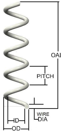
Round Wire Auger
