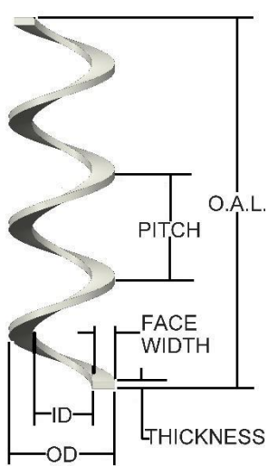
Flat Face Auger
